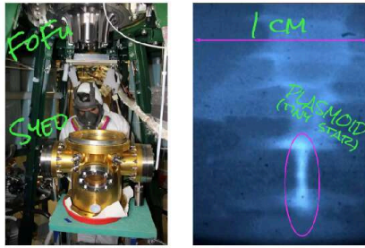
Left: Syed working under Focus Fusion Experimental Device; FoFu - nickname for Focus Fusion; Right: ICCD image of Plasmoid, colored.
